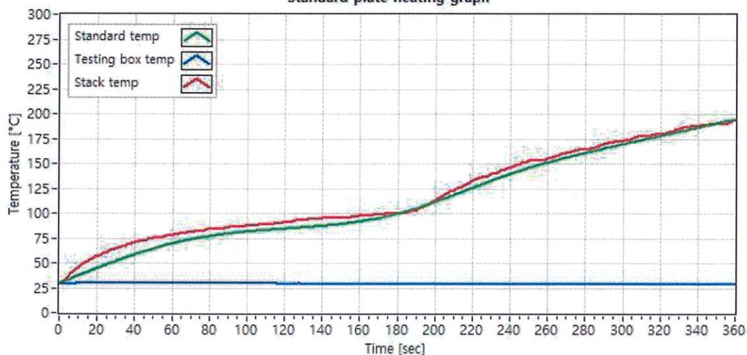
Standard plate heating graph
